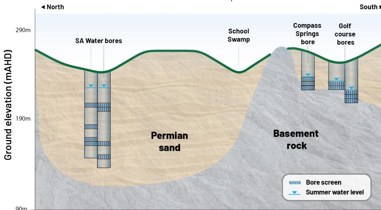
Fig. 5. Simplified north-south stratigraphic cross-section of Mount Compass area
