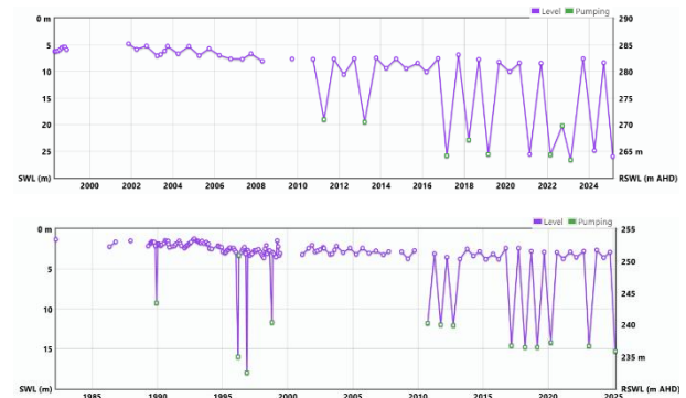
Fig. 3. Groundwater level in monitoring well NGK34 (top) located at the golf course, and NGK3 (bottom), located near the SA Water TWS bores
