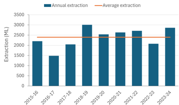
Fig. 2. Groundwater extraction from the Tookayerta Permian Groundwater Management Zone
